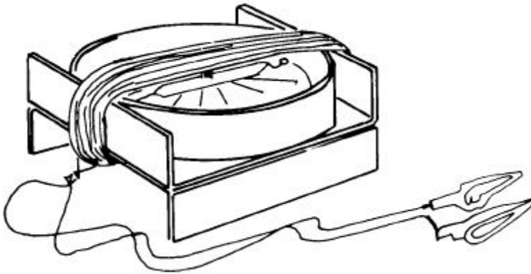
Diagram 2: Galvanometer
